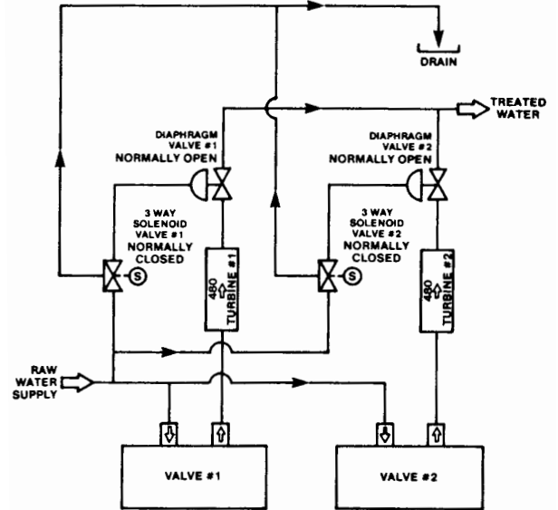
Multiple Tank System E/2 Flow Diagram
