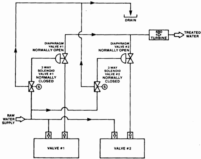
Multiple Tank System D/2 Flow Diagram
