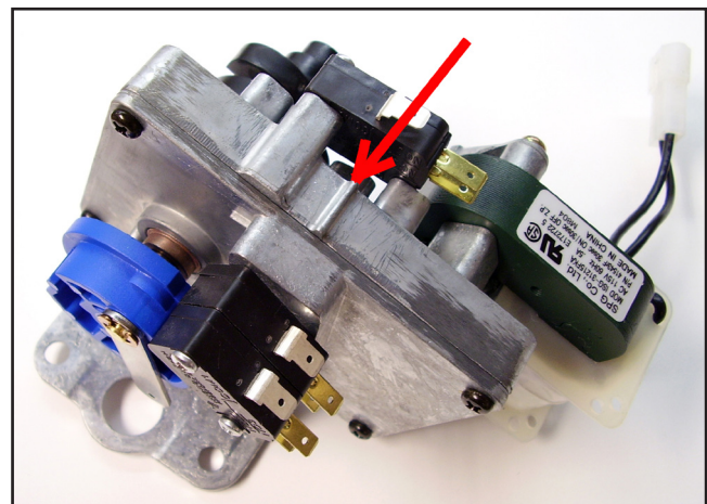
New Motor without Microswitch Insulators & Spacer Washers (red arrow shows new identifying mark)
