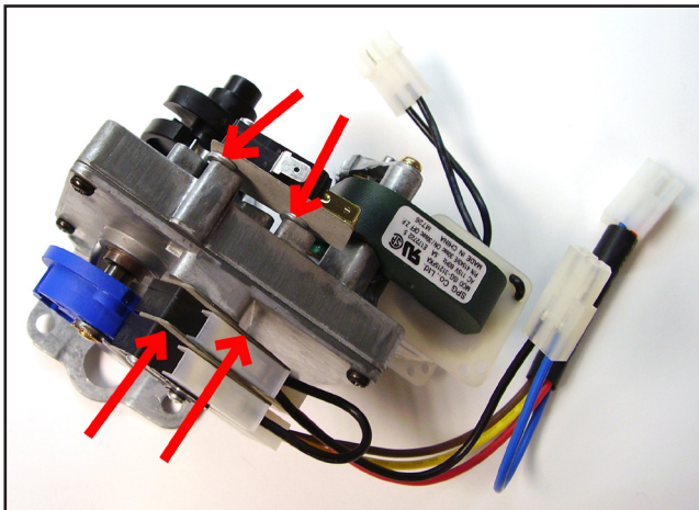
Old Motor with Microswitch Insulators & Spacer Washers (see red arrows)
