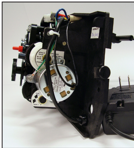
New Assembly (Motor, Ground Plate, & Label)
