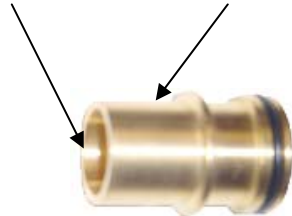
41242-01 Brass Connector, 1" & 1 1/4"- Sweat (W/O-ring)
